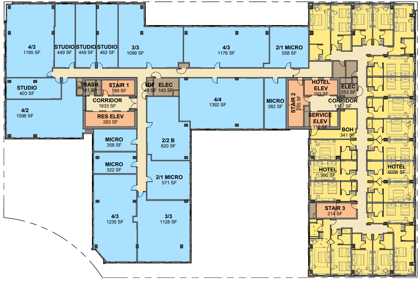
PROPOSED UPDATED FLOORPLAN
