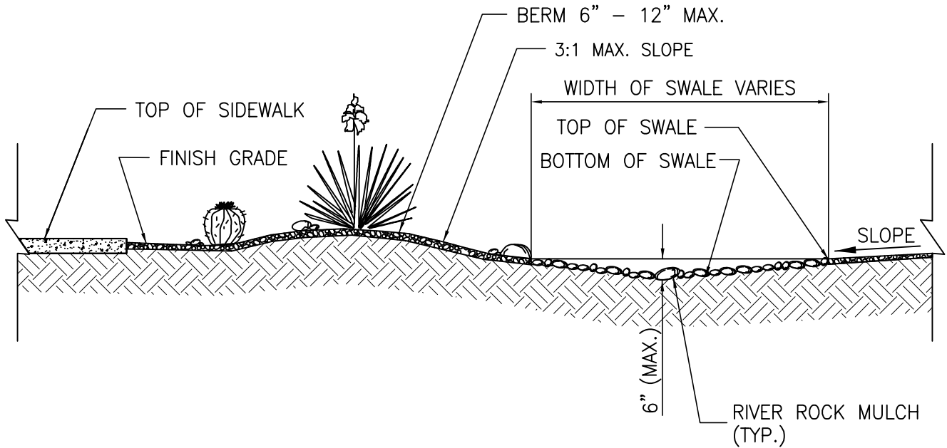
C-C SECTION THRU SWALE NTS
