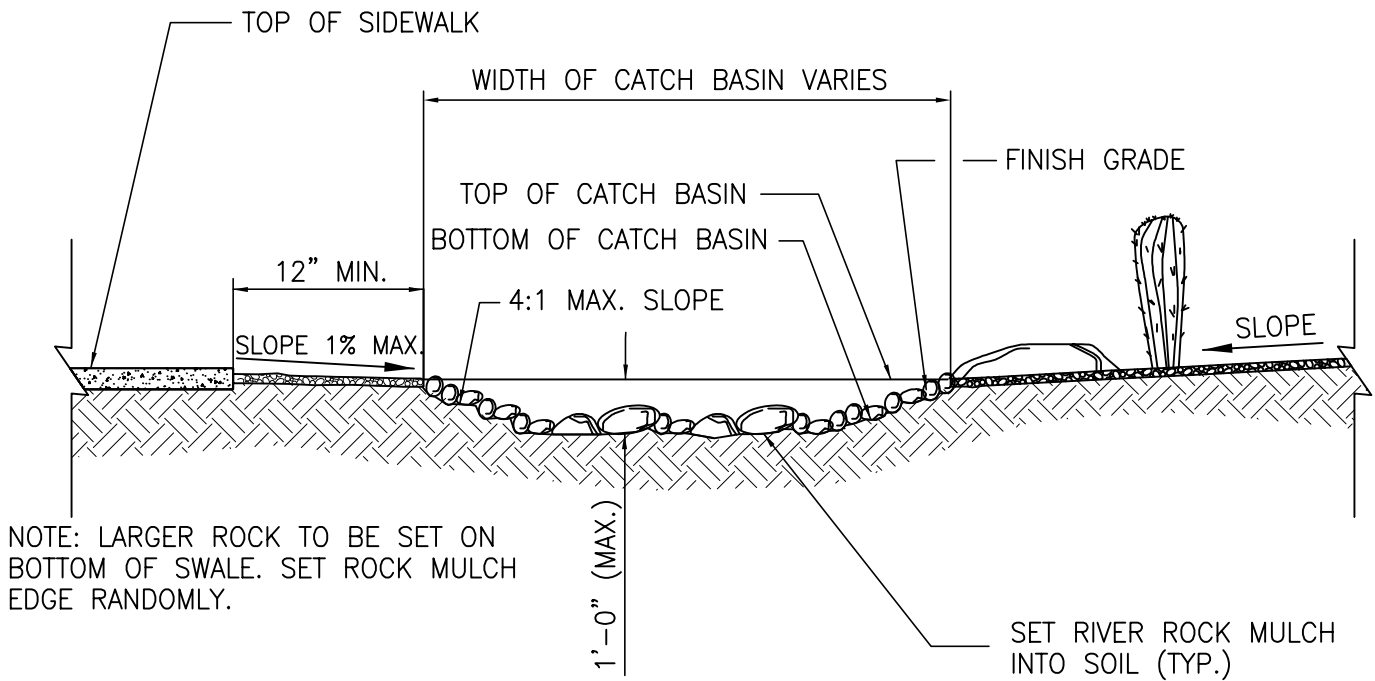
B-B SECTION THRU CATCH BASIN NTS
